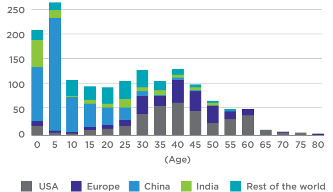
Figure 8: Investment in coal-fired power (Installed capacity - gigawatts)
